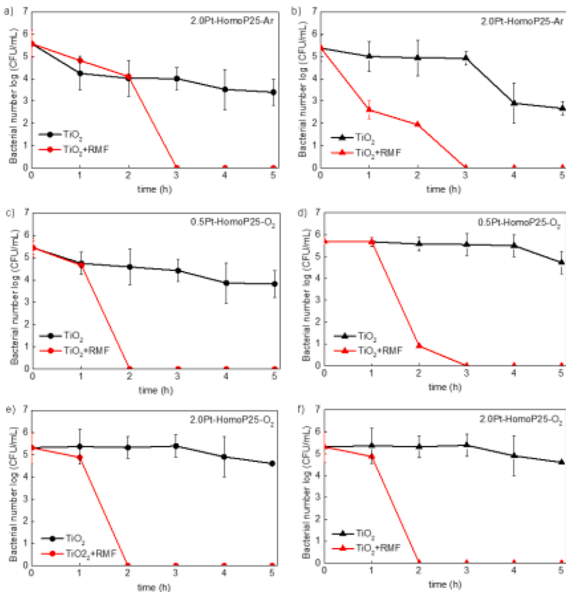
Fig. 10. The influence of the platinum-modified HomoP25 and RMF with indicated frequencies on the growth of E. coli (b, d, f) and S. epidermidis (b, e, f): 2.0Pt-HomoP25-Ar (a-b), 0.5Pt-HomoP25-O 2 (c-d), 2.0Pt-HomoP25-O 2 (e-f).
